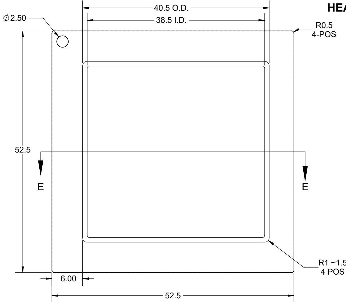
DETAIL F
