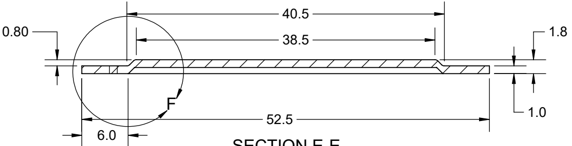
SECTION E-E
